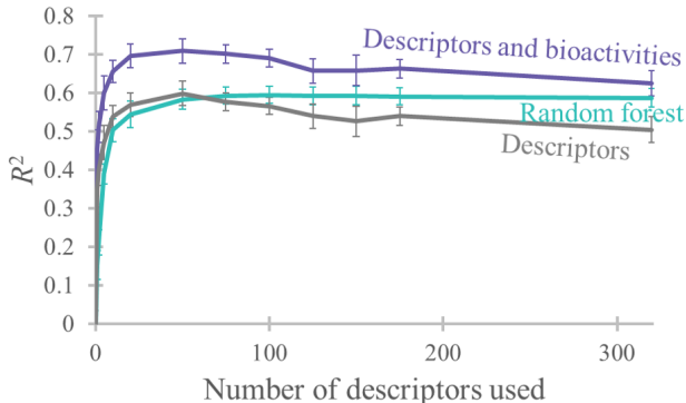
Figure 3: The coefficient of determination for predicting the activity of the adrenergic receptors with number of chemical descriptors. The magenta line is when the neural network is trained with both the activities and descriptors present, the grey line with just the descriptors, and the cyan line is for random forest. Error bars represent the standard error in the mean R^2 over five-fold cross-validation.
