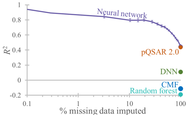
Figure 4: The coefficient of determination for predicting the activity of the clustered Kinase data set with percentage of data predicted. The cyan point is for the random forest approach, the blue point is the collective matrix factorisation (CMF) method, the dark green point is the deep neural network (DNN) approach, the orange point is the profile-QSAR 2.0 method, and the magenta line is the neural network proposed in this work. The magenta line shows that the accuracy of the neural network predictions increases when focussing on the most confident predictions, at the expense of imputing only a proportion of the missing data. This confirms that the reported confidences in the predictions correlate strongly with their accuracy. Error bars represent the standard error in the mean R^2 value over all 159 assays, and where not visible are smaller than the size of the points.
