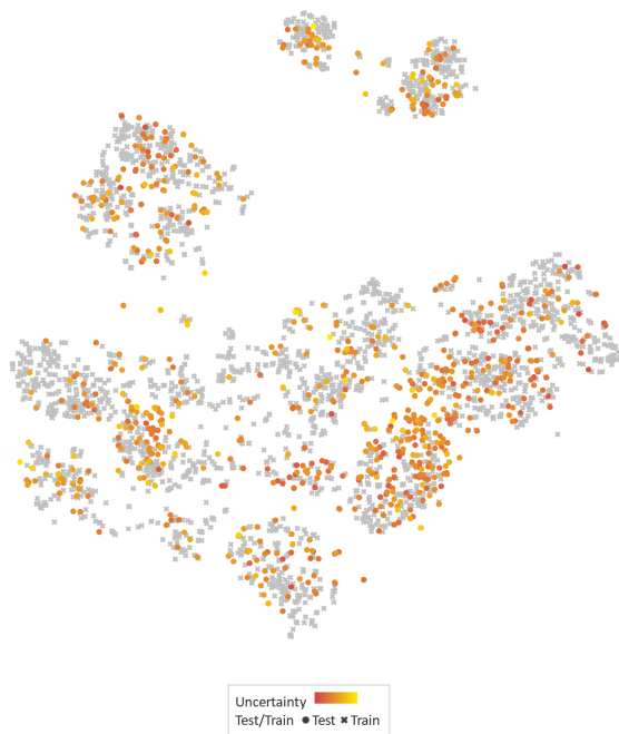
Figure 6: A 2-dimensional t-SNE embedding of the input descriptor space for ChEMBL assay 688660. The grey crosses show the training data and the coloured points show the test data with colour indicating the uncertainty estimate of the network in its predictions, where red indicates zero uncertainty and yellow a high uncertainty of 1 log unit.
